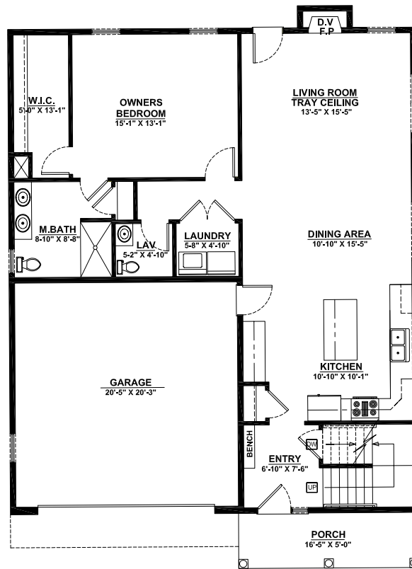
FIRST FLOOR PLAN (1218 s.f.) GARAGE (439 s.f.)
