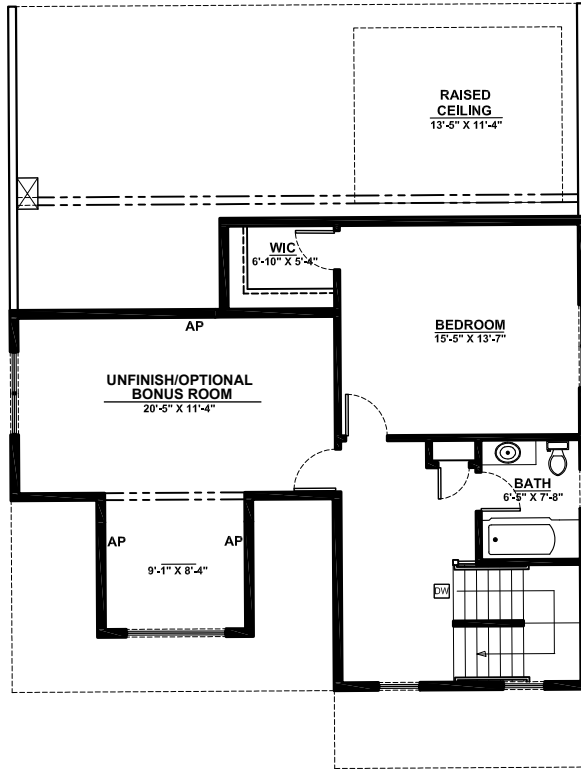
SECOND FLOOR PLAN (545 s.f.) s.f. does not include Bonus Room
