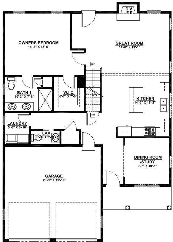
FIRST FLOOR PLAN (1223 s.f. GARAGE 418 s.f.)
